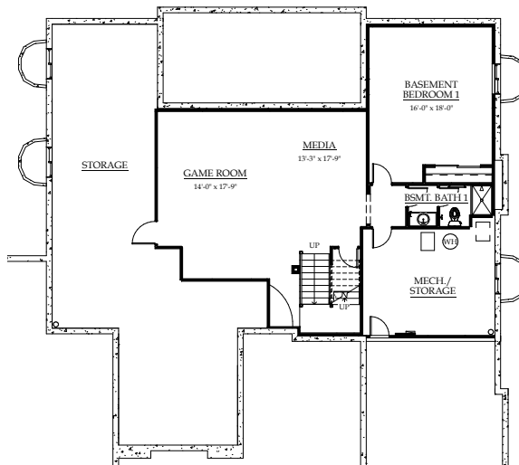
FINISHED BASEMENT WITH ADDITIONAL BEDROOM & BATH
