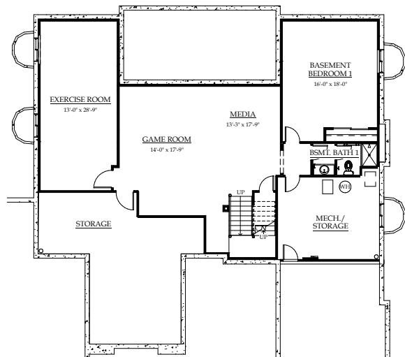
FINISHED BASEMENT WITH ADDED EXERCISE ROOM
